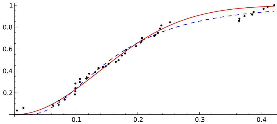
Figure 2: The empirical distribution for the distance function (??), together with a fitted \chi -distribution (drawn solid) and a fitted log-normal distribution (drawn dashed), found by solving the nonlinear least squares problems (??) and (??).
